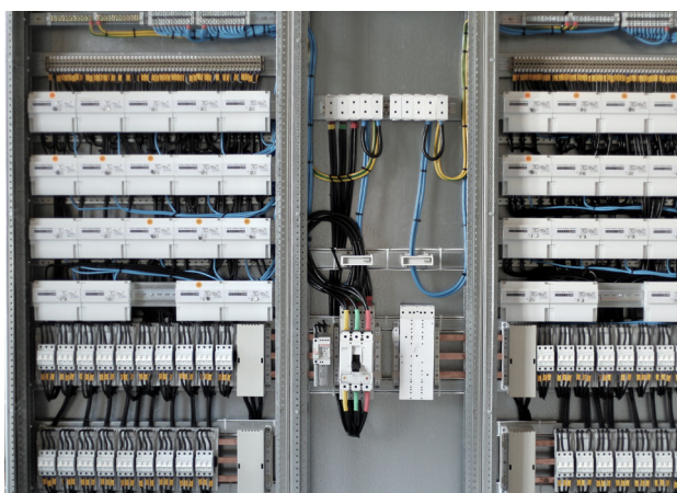
Control cabinet
