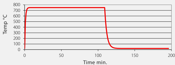
Heating and cooling times tubular Ø 8.5mm
